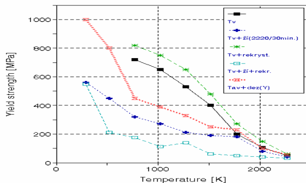
Fig.5 Dependence of tungsten's yield strength on temperature
