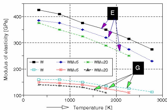
Fig.4 Dependence of modulus of elasticity in tension (E) and in shear (G) on temperature
