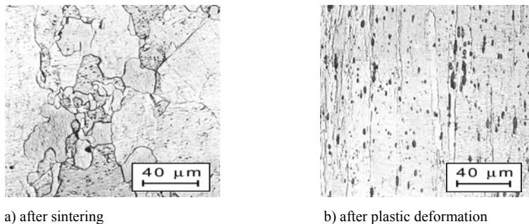
Fig.3 The change of microstructure WThO 2 after sintering and wire drawing
