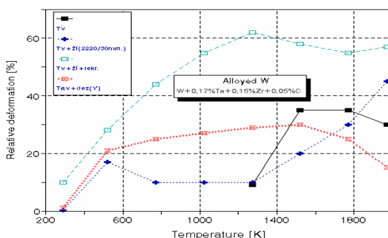
Fig.6 Dependence of tungsten's ductility on temperature and production technology [5]
