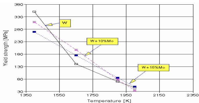
Fig. 1 Dependence of ultimate strength of the W-Mo type alloy on the temperature
