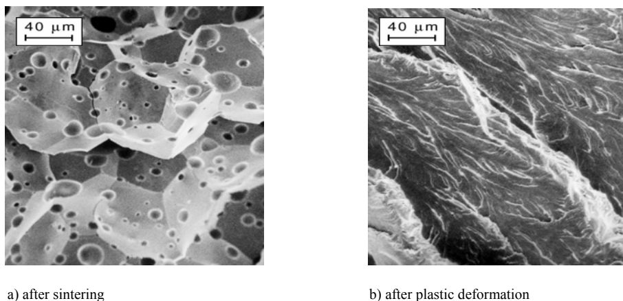
Fig.2 Shows the microstructure and fracture surface on WThO_2 sample
